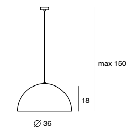
Dome Pendant M SQ-360MP E27 1 x Max 46W Ribbed reflector bulb cover
