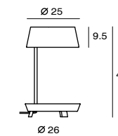
Carry Table SQ-6353MDU E27 1 x Max 46W On/off rocker switch USB charger
