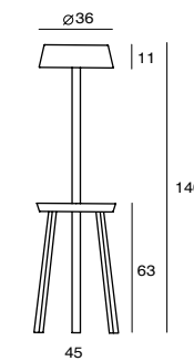
Carry Floor SQ-6350MFU E27 2 x Max 46W On/off rocker switch USB charger
