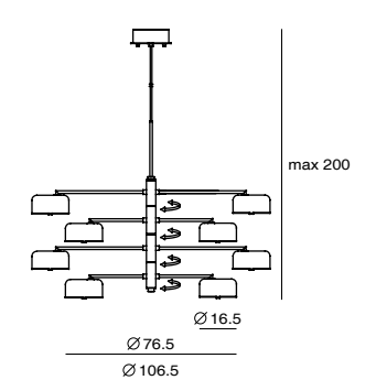
Lalu+ Pendant P8 SLD-2501MPR8 LED 8 x 5W (2700K CRI 90, 3600lm) Rotatable cross bar Black textile wire
