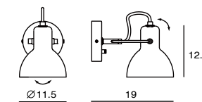
Laito Opal Wall SQ-793WR E14 1 x Max 25W Shade rotatable On/off rotary switch Black textile wire Materials : mouth-blown glass, steel Color : matt opal shade + matt brass body Canopy : Type A43, matt white Back Plate : Type B3
