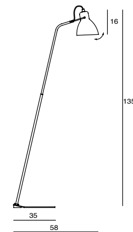
Laito Opal Floor SQ-893FB E27 1 x Max 46W Shade rotatable On/off foot switch Black textile cord Materials : mouth-blown glass, steel Color : matt opal shade + matt brass body + matt white base
