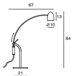
Hercules Table SLD-79DTE LED 8.6W (3000K, CRI 90, 730lm) Shade rotatable Arm adjustable Touch dimmer switch Black textile cord Material : steel Color : copper shade + matt black body matt brass shade + matt black body
