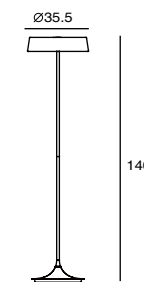
China LED Floor SLD-6354MFE LED 18W (2700K, CRI 90, 1900lm) Adaptor driver Foot dimmer Black textile cord
