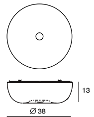
Cloud Ceiling SLD-7938C LED 30W (2700K, CRI 90, 940lm) Built-in dimmable driver
