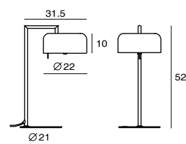
Lalu+ Table SQ-250MDR E27 1 x Max 46W Dip switch Shade rotatable Black textile cord
