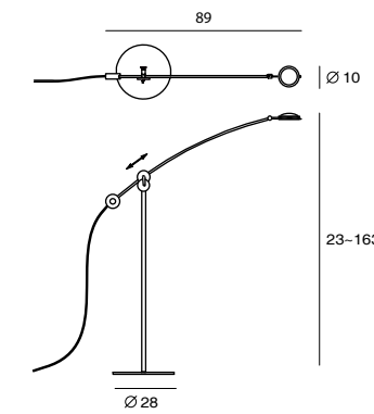
Planet Floor SLD-100FRTE LED 8.6W (3000K, CRI 90, 600lm) Multi- Direction adjustable Touch dimmer swtich, adaptor driver Black textile cord
