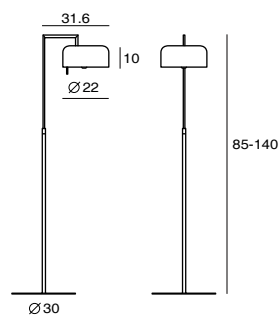
Lalu+ Floor SQ-250MFR E27 1 x Max 46W Dip switch Shade rotatable Height adjustable Black textile cord
