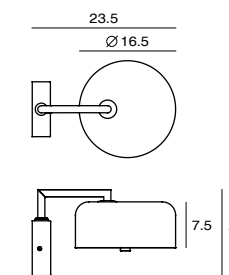
Lalu+ Wall SLD-2501MWRTE LED 5W (2700K CRI 90, 425lm) Shade rotatable Touch dimmer switch
