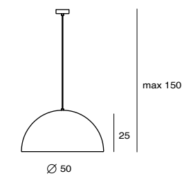
Dome Pendant L SQ-3650MP E27 1 x Max 46W Ribbed reflector bulb cover
