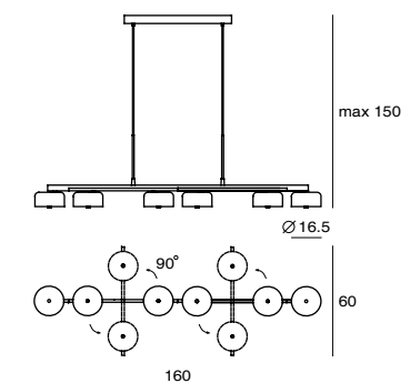
Lalu+ Pendant PL6 SLD-2501MCTR6 LED 6 x 5W (2700K CRI 90, 2700lm) Rotatable cross bar Black textile wire
