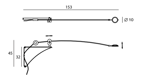
Planet Wall SLD-100WRTE LED 8.6W (3000K, CRI 90, 600lm) Multi- Direction adjustable Touch dimmer swtich, adaptor driver Black textile cord
