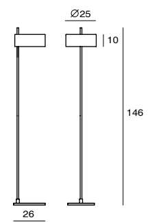
Re Lalu Floor SQ-250FW E27 1 x Max 46W Push on/off switch Black textile cord
