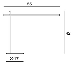
Ticktock Table SLD-393DP6 LED 6 x 1W (3000K, CRI80, 540lm) Push on/off switch adaptor driver Red textile cord
