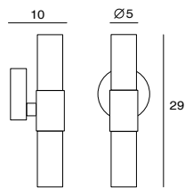
T1 Wall 2 SG-50WB2 G9 2 x Max 40W/ 3W LED
