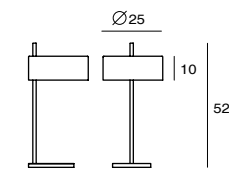
Re Lalu Table SQ-250DW E27 1 x Max 46W Push on/off switch Black textile cord
