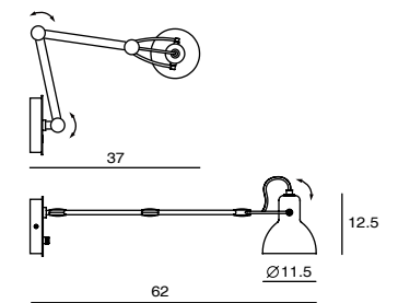
Laito Opal Wall L SQ-793WA E14 1 x Max 25W Shade & arm rotatable On/off rotary switch Black textile wire Materials : mouth-blown glass, steel Color : matt opal shade + matt brass body Canopy : Type A14, matt white Back Plate : Type B4
