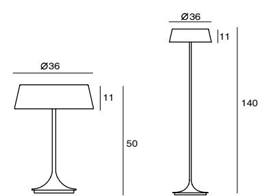
China Table SQ-6350MDJ2 E27 2 x Max 46W DJ dimmer Black textile cord
