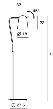
Dodo Floor SQ-218FR E27 1 x Max 46W Shade rotatable Dip switch Black textile cord
