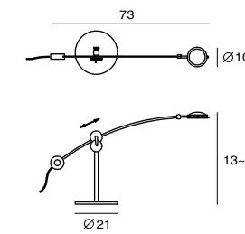
Planet Table SLD-100DRTE LED 8.6W (3000K, CRI 90, 600lm) Multi- Direction adjustable Touch dimmer swtich, adaptor driver Black textile cord
