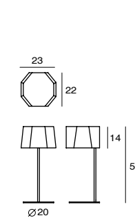
Zhe Table SQ-2322MD E27 1 x Max 46W Red textile cord
