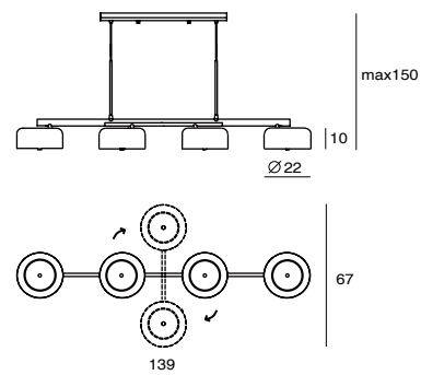
Lalu+ Pendant PL4 SQ-250MCTR4 E27 4 x Max 46W Rotatable cross bar Black textile wire
